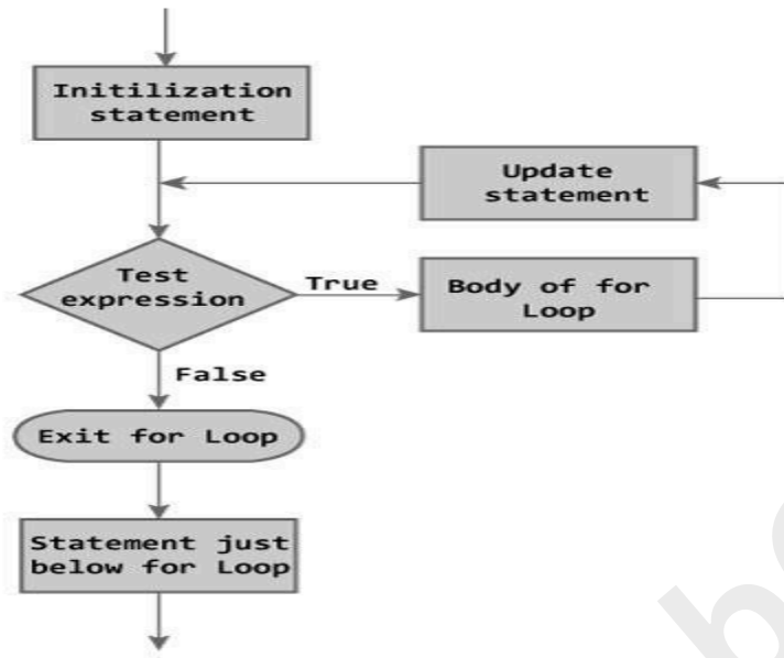
Figure: Flowchart of for Loop
